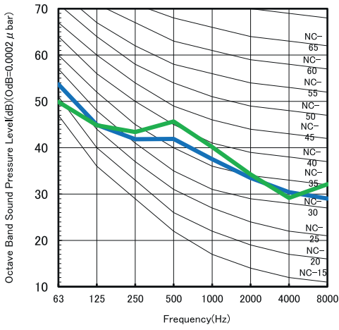
CU-Z25CKE (Cooling)
