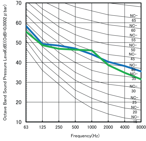
CU-Z35CKE (Heating)
