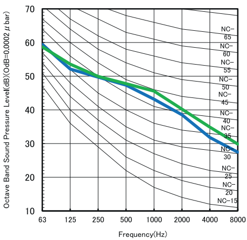
CU-Z71CKE (Cooling) Octave Band Central Frequency(Hz)
