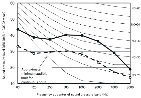
CS-Z50CKEW (Cooling) Octave Band Central Frequency(Hz)
