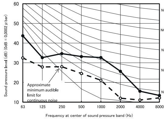
CS-Z25CKEW (Heating) Octave Band Central Frequency(Hz)
