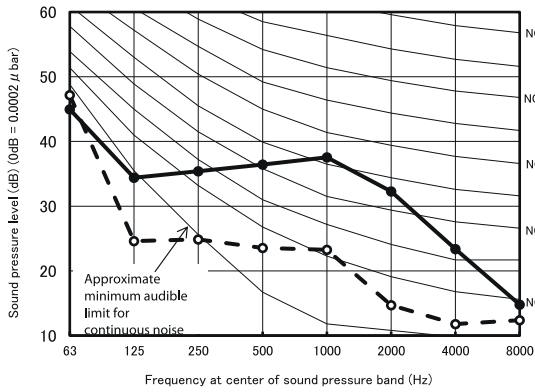
CS-Z35CKEW (Cooling) Octave Band Central Frequency(Hz)
