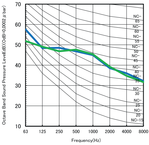
CU-Z50CKE (Cooling) Octave Band Central Frequency(Hz)
