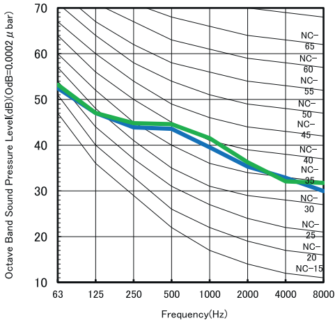
CU-Z35CKE (Cooling)
