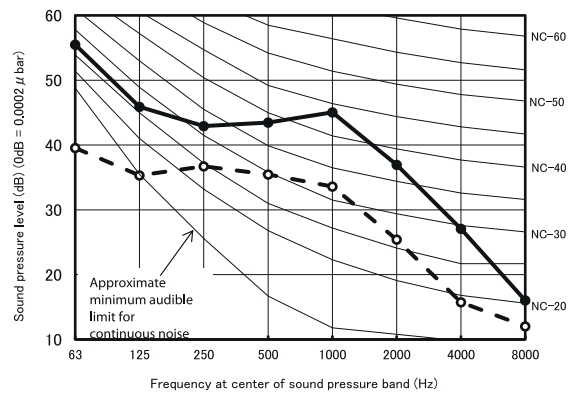
CS-Z71CKEW (Heating) Octave Band Central Frequency(Hz)
