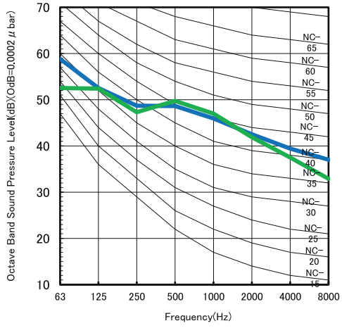
CU-Z50CKE (Heating) Octave Band Central Frequency(Hz)
