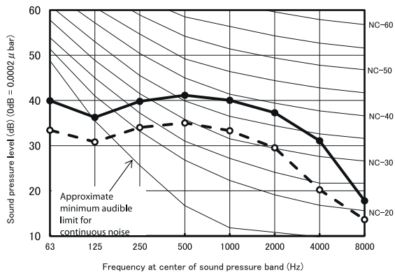
CS-Z71CKEW (Cooling) Octave Band Central Frequency(Hz)
