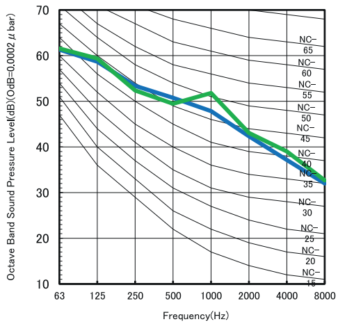
CU-Z71CKE (Heating) Octave Band Central Frequency(Hz)
