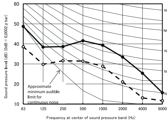
CS-Z35CKEW (Heating) Octave Band Central Frequency(Hz)
